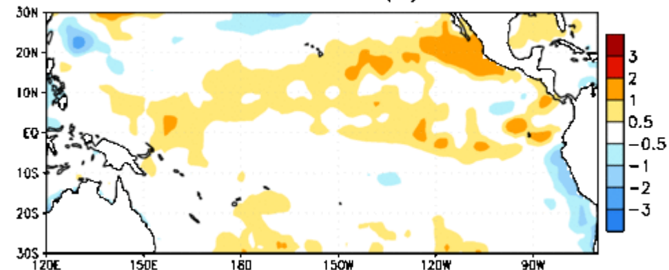
Week centered on 18 JUL 2018 SST Anomalies (°C)
